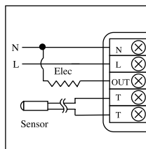
(3) Electrical Heating
