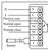
(1) Passive Wall-boiler
